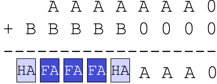
Figure 5.2: Adder hardware requirements
