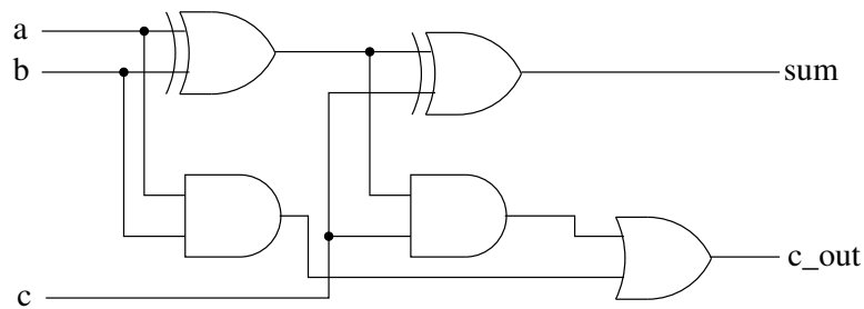
Figure 3.2: A single bit slice of a full-adder
