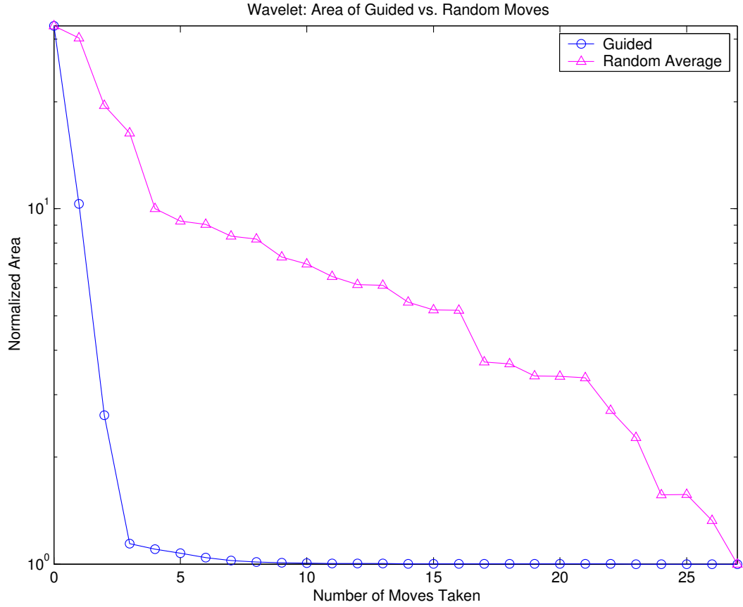
Figure 4.8: Wavelet area vs. number of optimization steps implemented
