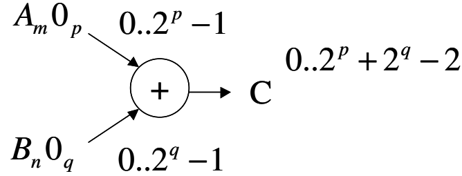
Figure 5.7: Error model of an adder
