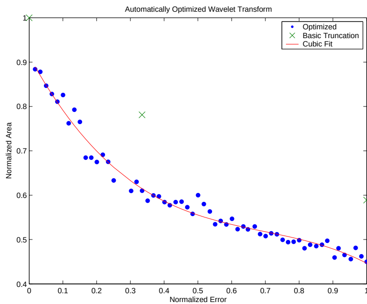
Figure 5.19: Optimized results for wavelet transform
