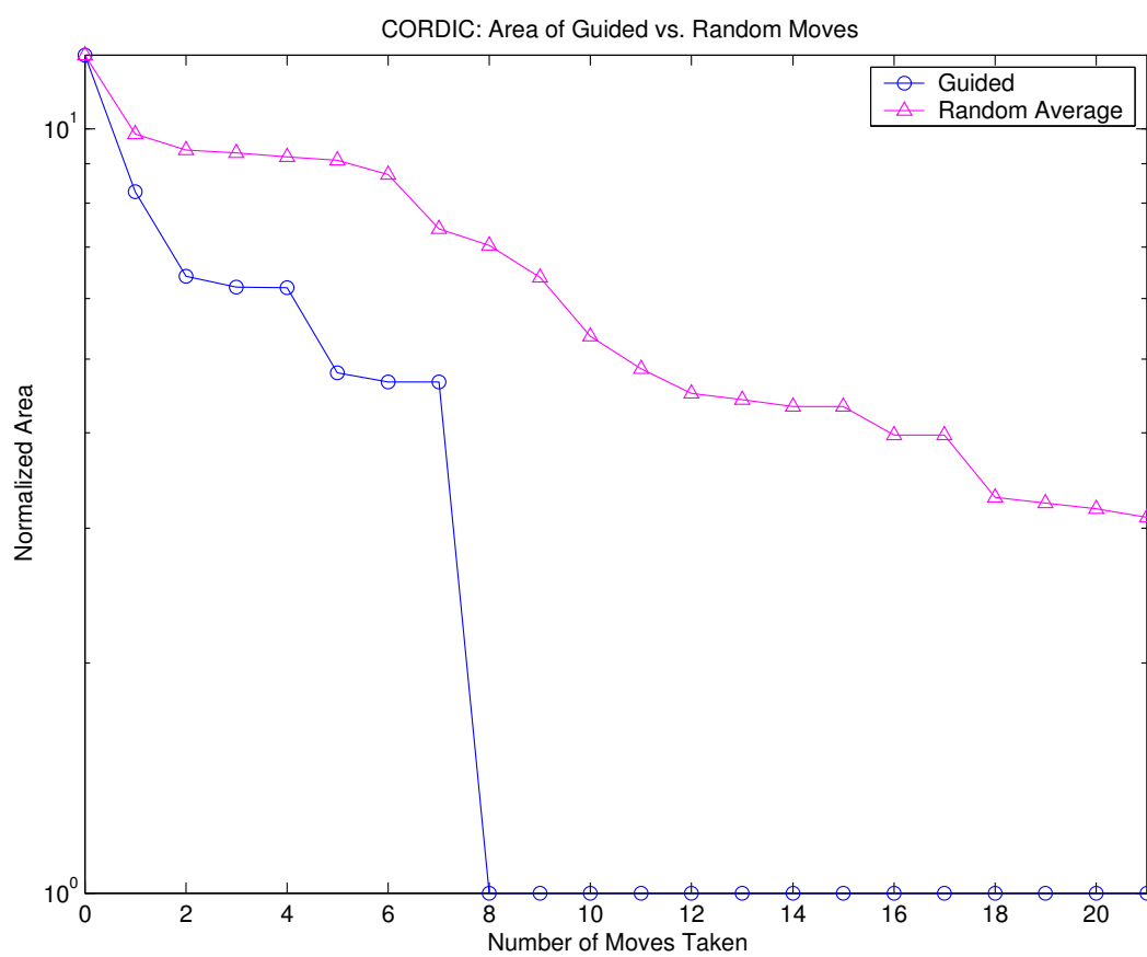
Figure 4.9: CORDIC benchmark results
