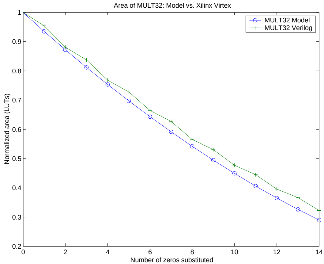
Figure 5.6: Multiplier model verification
