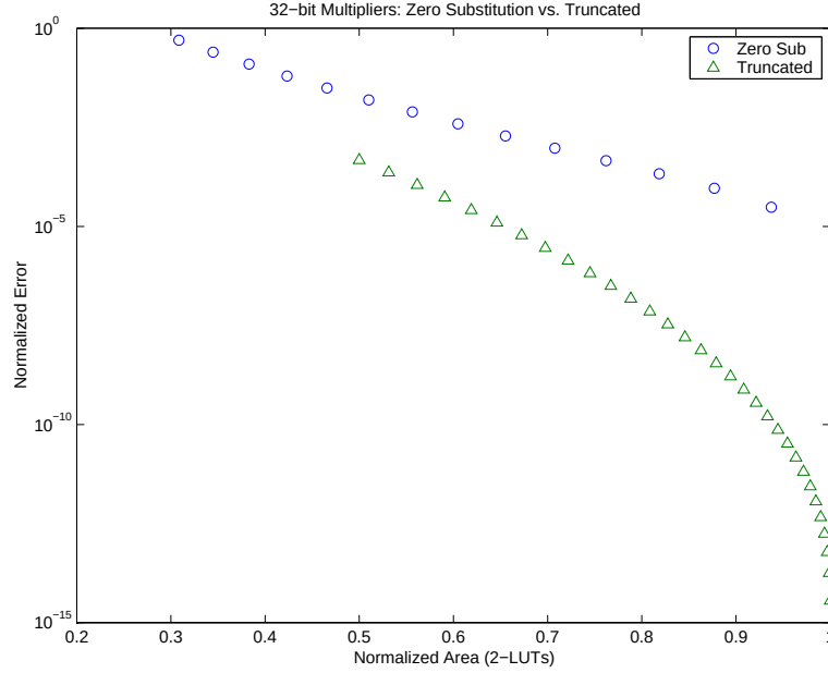
Figure 5.17: Error to area profile of zero-substitution 32-bit multiplier and truncated 32-bit multiplier
