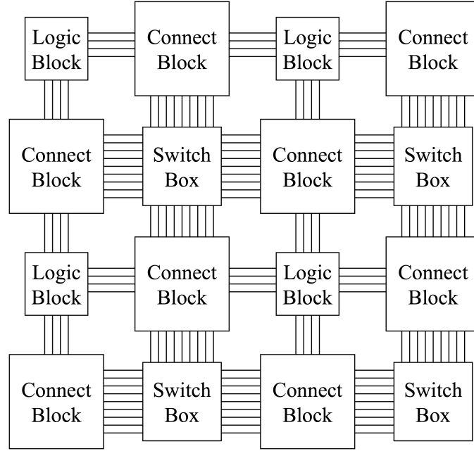
Figure 2.1: Typical island-style FPGA routing structure
