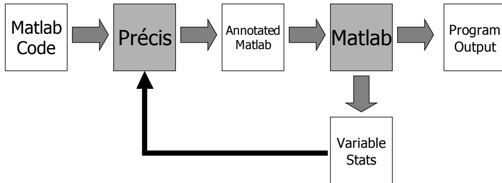
Figure 4.5: Development cycle for range finding analysis
