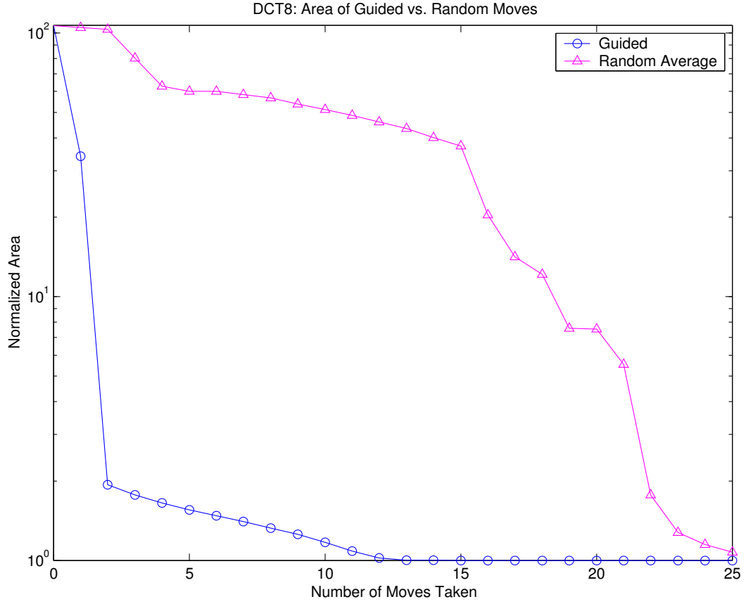
Figure 4.11: 8-point 1-D DCT results
