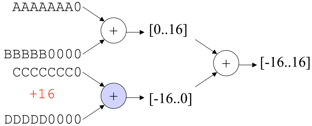
Figure 5.15: Simple three adder data path after renormalization has maximum error range of 16
