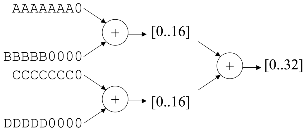
Figure 5.14: Simple three adder data path before renormalization has maximum error range of 32
