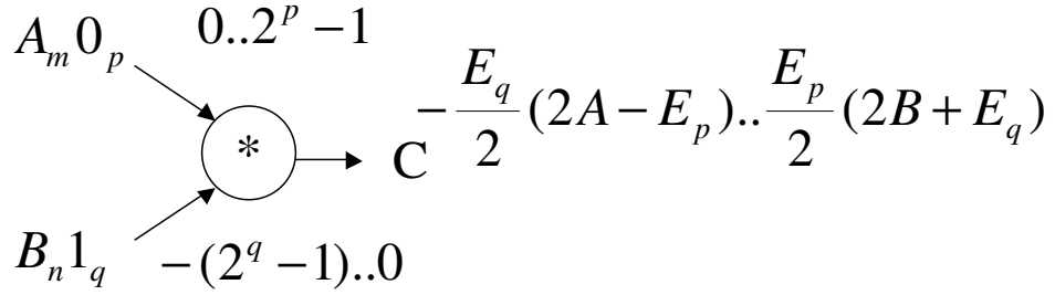
Figure 5.10: Normalized error model of a multiplier
