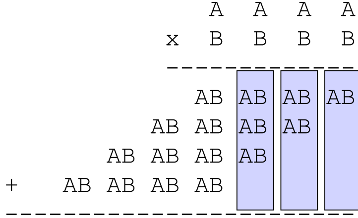
Figure 5.16: Truncated multiplier: removal of shaded columns reduces area and increases error
