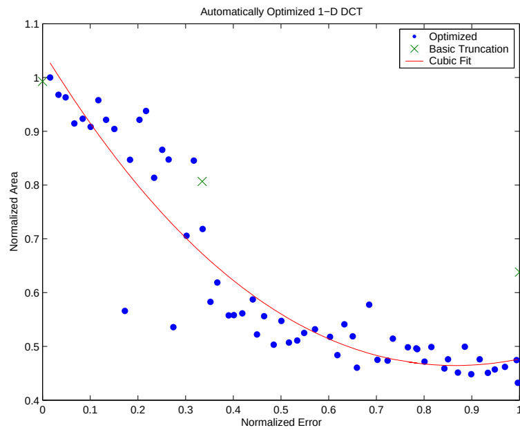
Figure 5.21: Optimized results for 1-D discrete cosine transform
