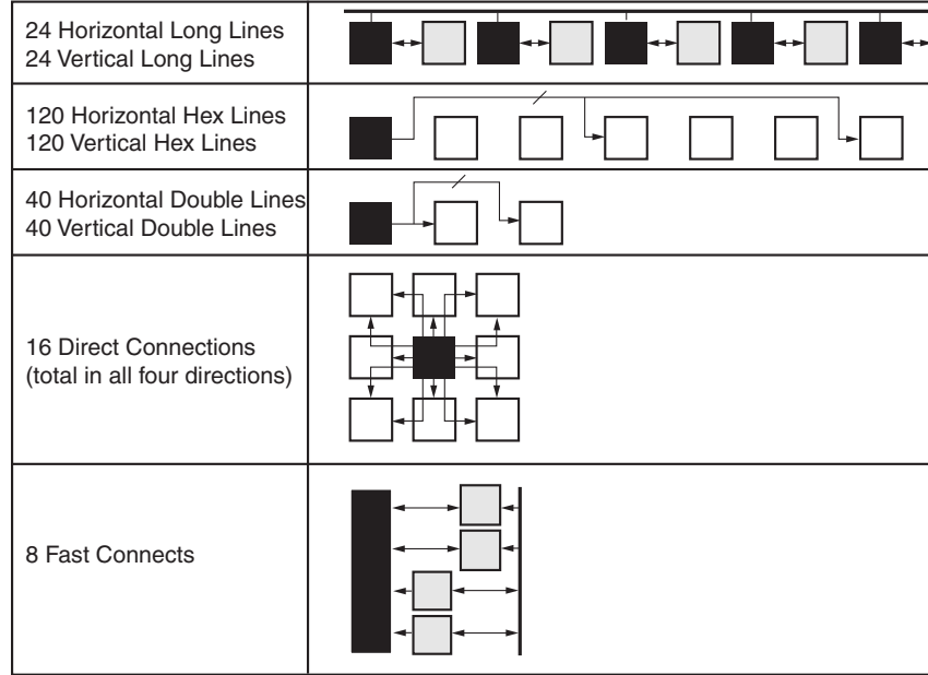
Figure 2.6: Xilinx Virtex-II routing detail [81]
