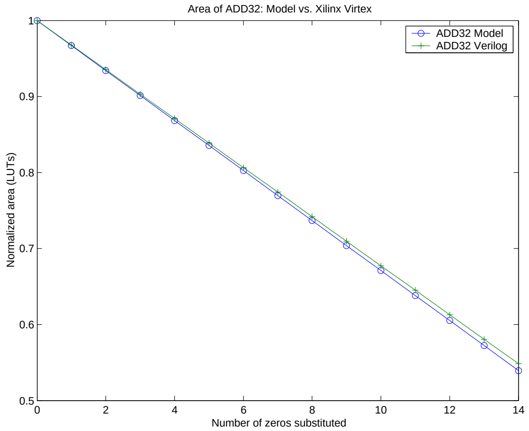
Figure 5.5: Adder model verification
