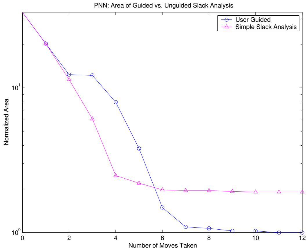
Figure 4.13: PNN area with user-defined variable precision ranges
