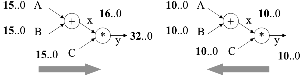
Figure 4.2: Simple propagation example
