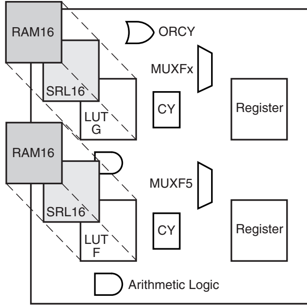
Figure 2.4: Xilinx Virtex-II Slice [81]
