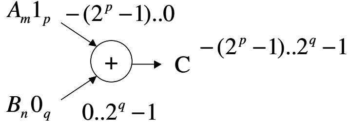
Figure 5.9: Normalized error model of an adder
