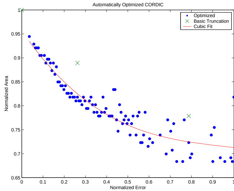
Figure 5.20: Optimized results for CORDIC
