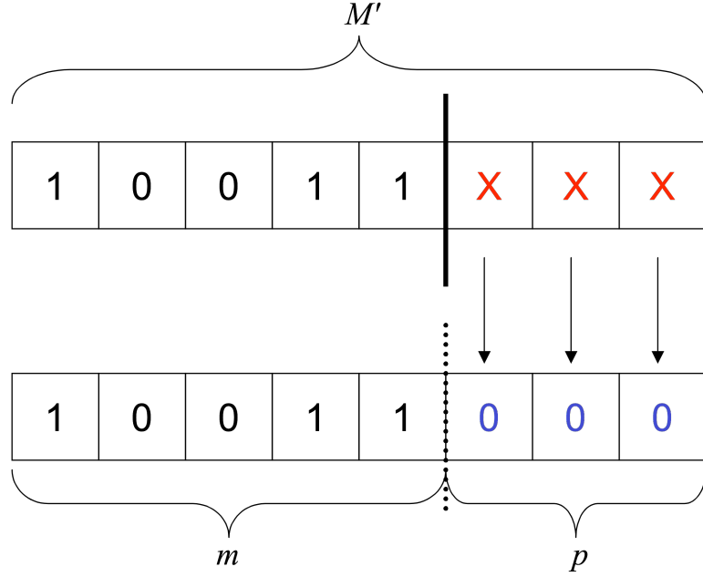
Figure 5.1: Constant substitution
