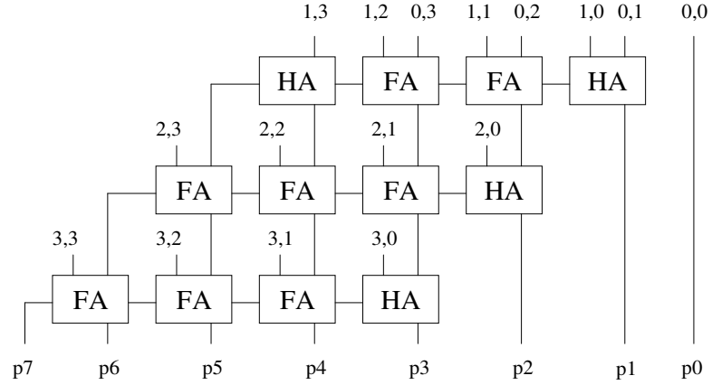
Figure 5.3: Multiplication structure
