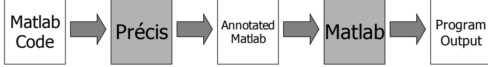
Figure 4.3: Flow for code generation for simulation
