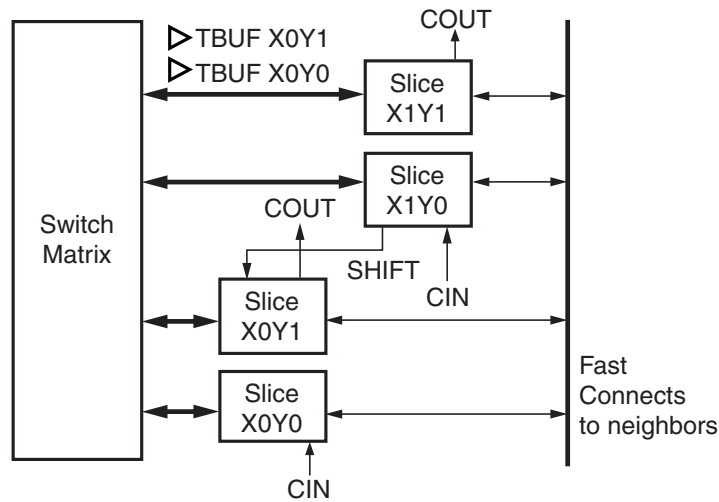
Figure 2.3: Xilinx Virtex-II Configurable Logic Block (CLB) [81]
