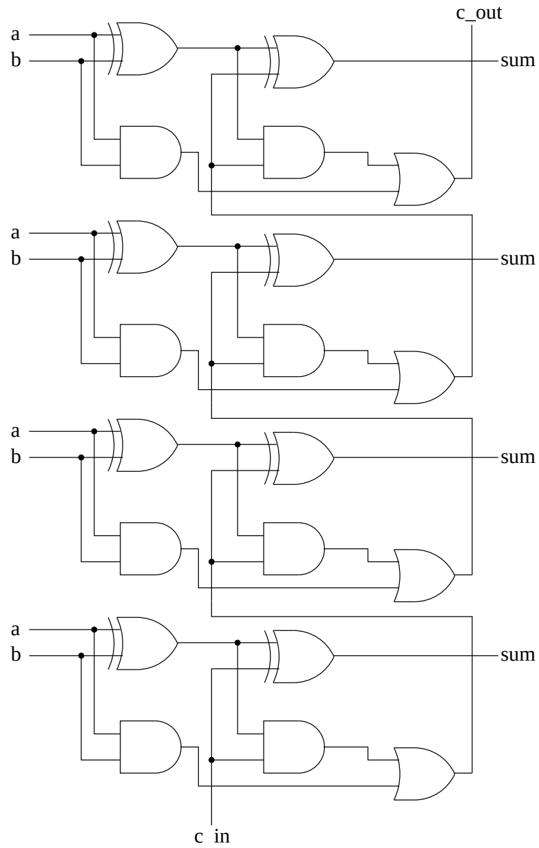
Figure 3.3: A four-bit adder built from four one-bit full-adders
