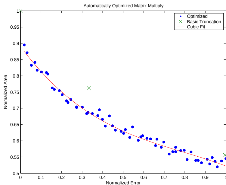
Figure 5.18: Optimized results for matrix multiply
