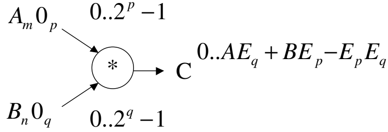
Figure 5.8: Error model of a multiplier
