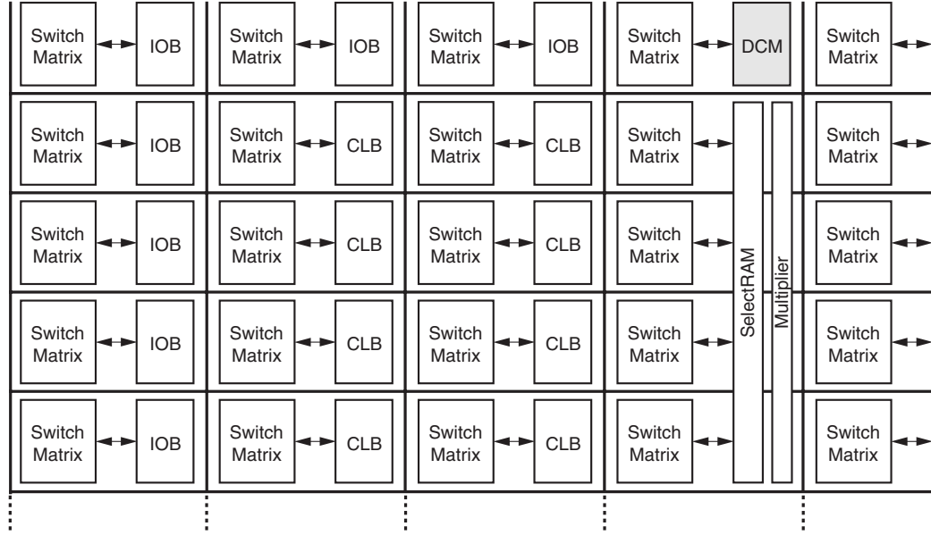
Figure 2.5: Xilinx Virtex-II global routing channels [81]
