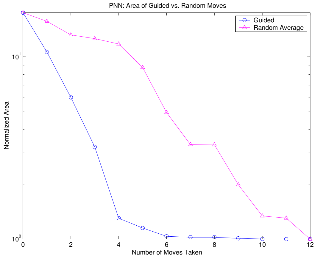
Figure 4.12: PNN area vs. number of optimization steps implemented utilizing only range-analysis-discovered values
