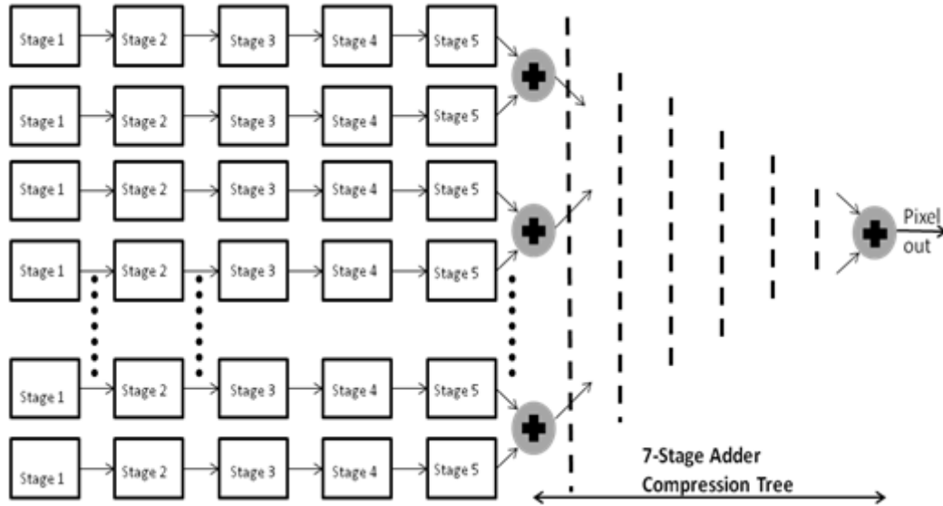
Figure 3.10 Pipelined and Parallel Data Path
