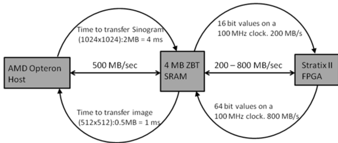
Figure 3.1: Data rates to Shared Memory
