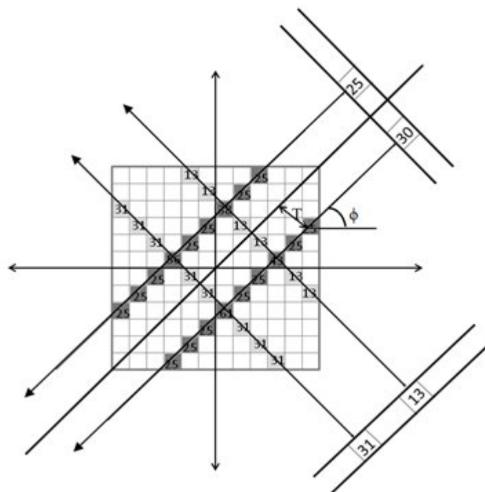
Figure 2.7 Backprojecting along rays
