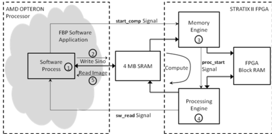
Figure 3.11 System Architecture
