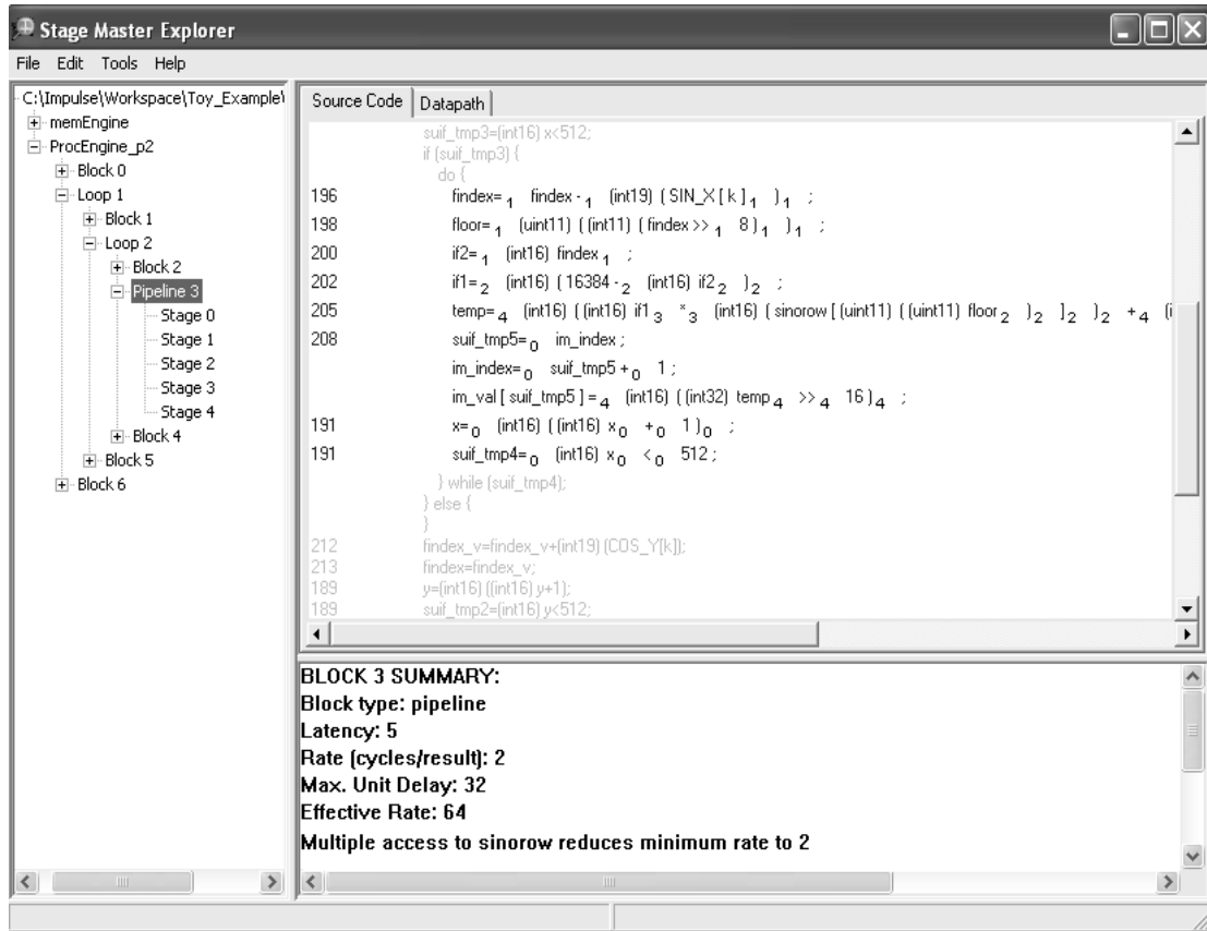
Figure 3.9 Impulse C Stage Master Explorer
