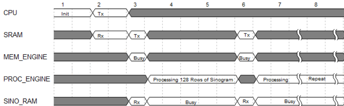
Figure 4.2 System timing for FPGA accumulation. Reconstruction from 512 projections
