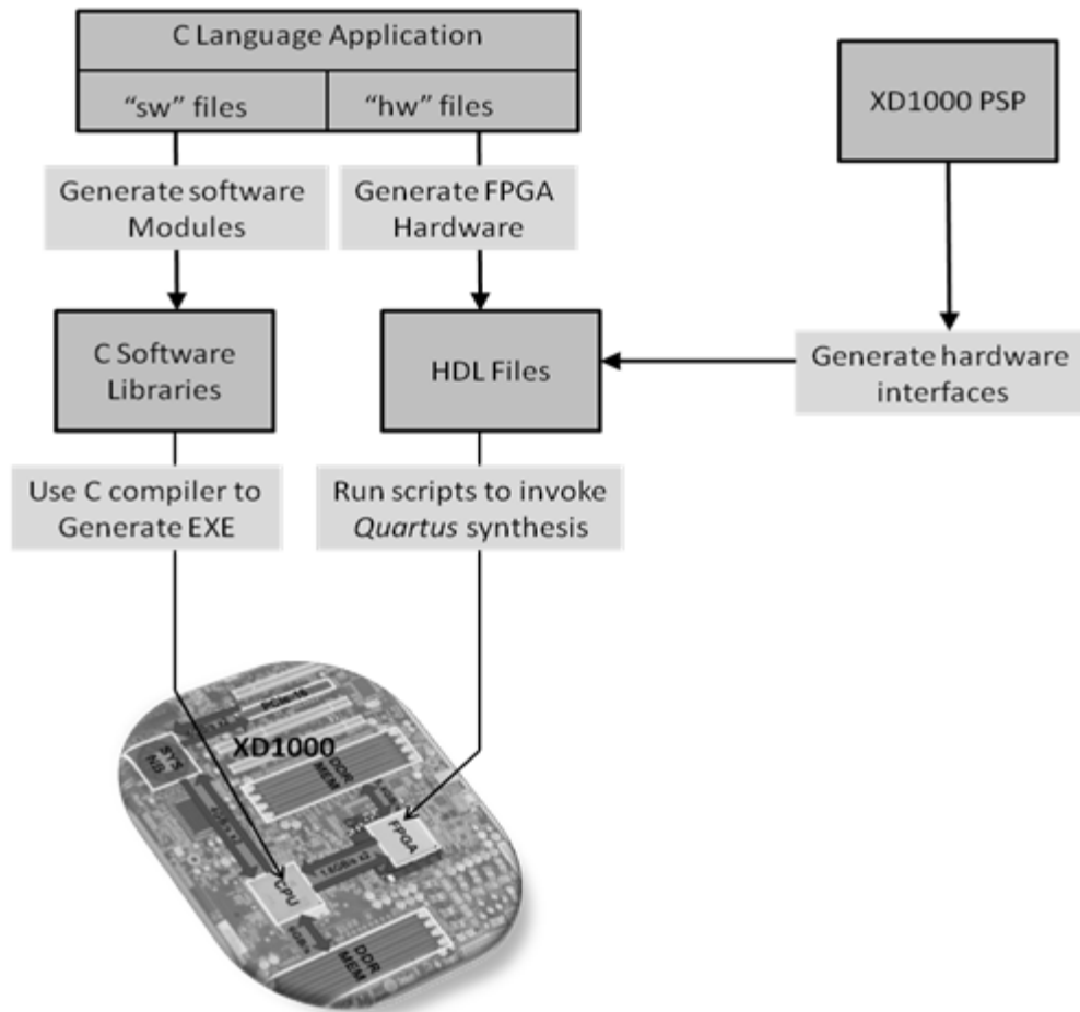
Figure 2.10 Design flow to target XD1000 with Impulse C
