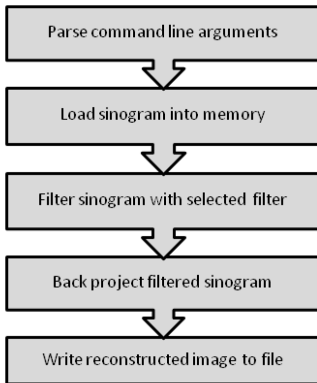
Figure 2.5 Flow of operations in software implementation of FBP
