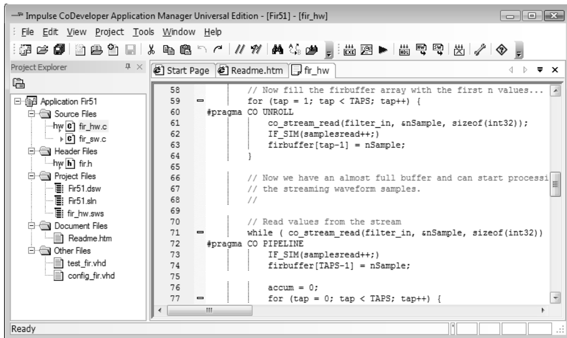
Figure 2.9 CoDeveloper Application Manager Screenshot
