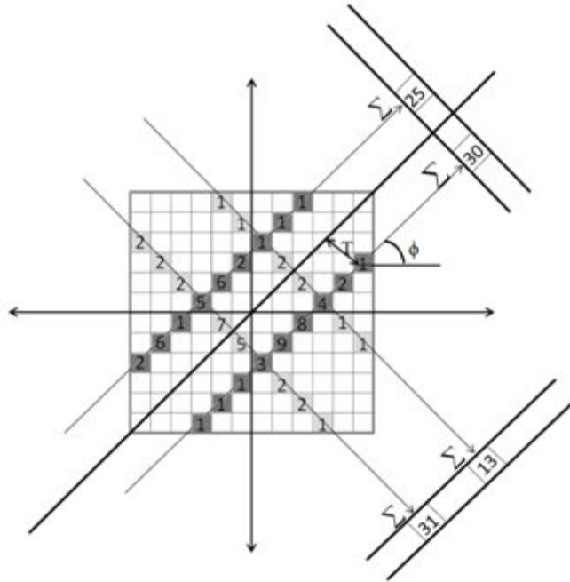
Figure 2.6 Image Pixels contributing to detector values
