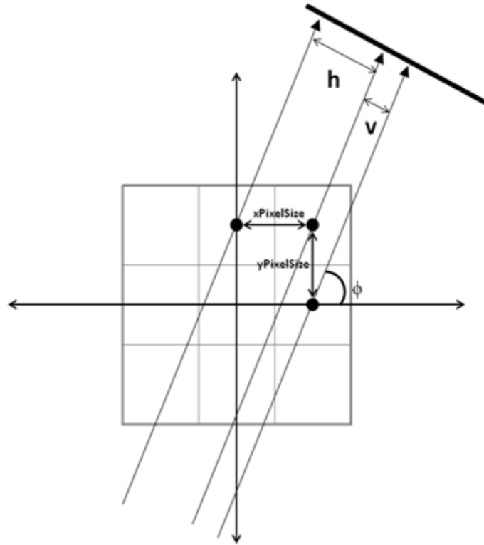
Figure 3.6 Detector offsets when walking through image
