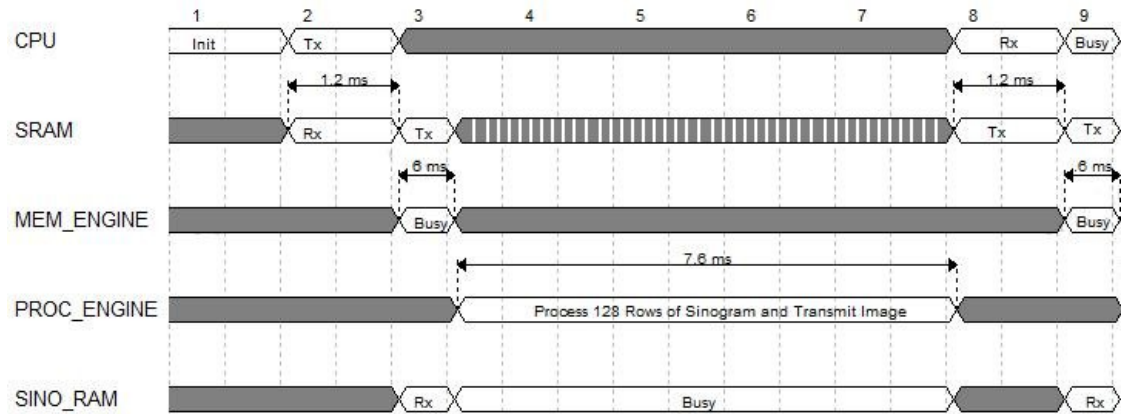
Figure 4.1 System timing for CPU accumulation. Reconstruction from 512 projections
