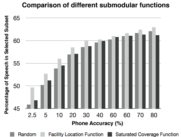
Figure 2: Phone accuracy obtained by random selection, facility location function, and saturated coverage function (string kernel similarity measure).
