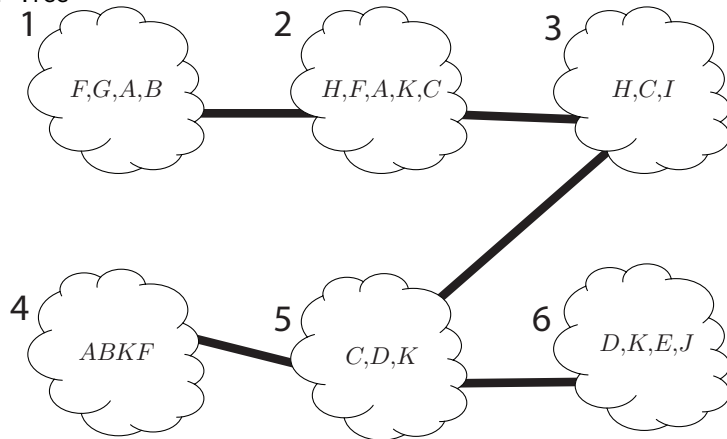
Cluster Tree
